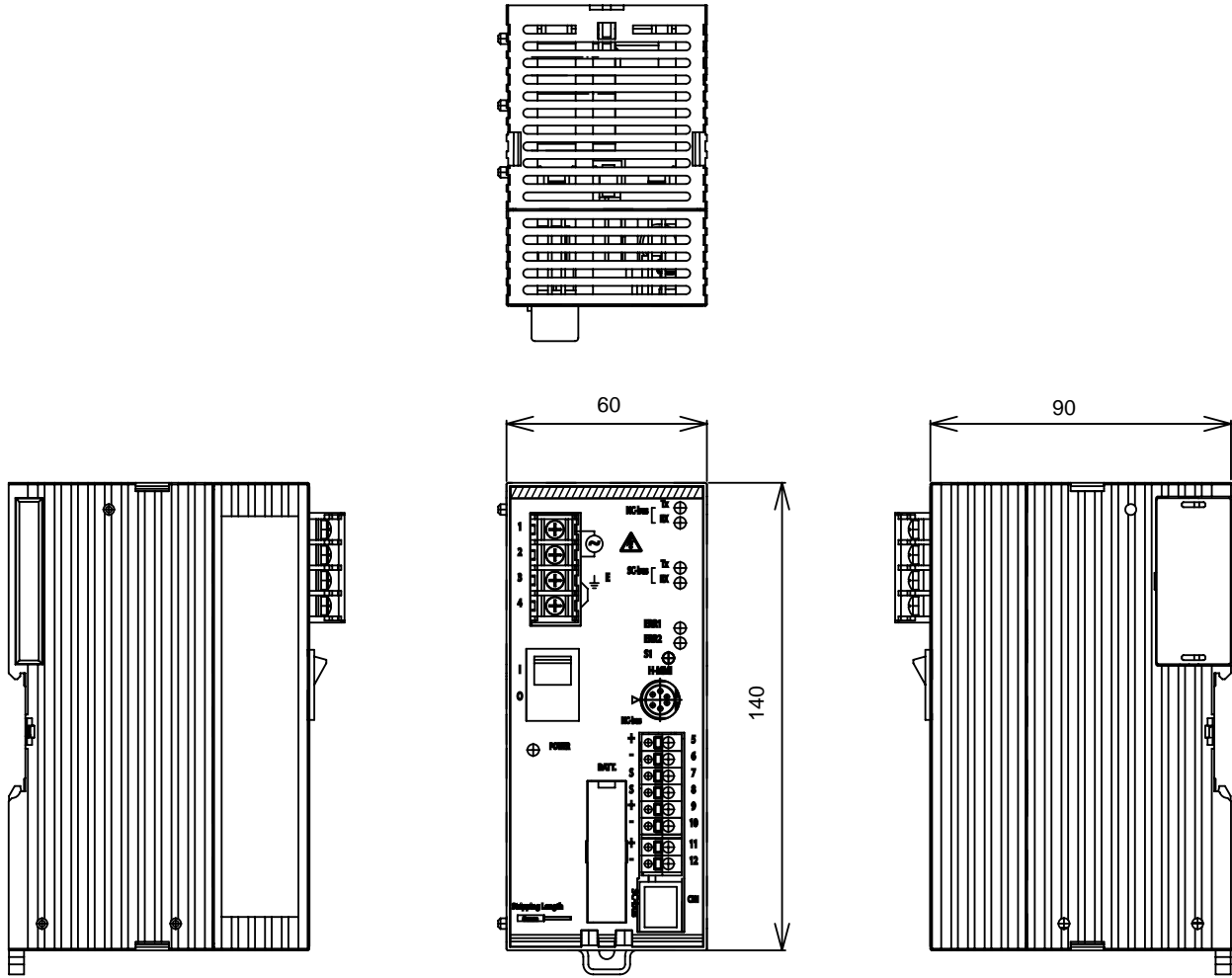
Figure 3. Dimensions (mm)
