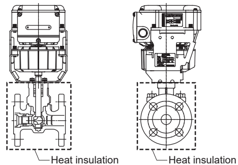
Figure 7 Heat insulation
