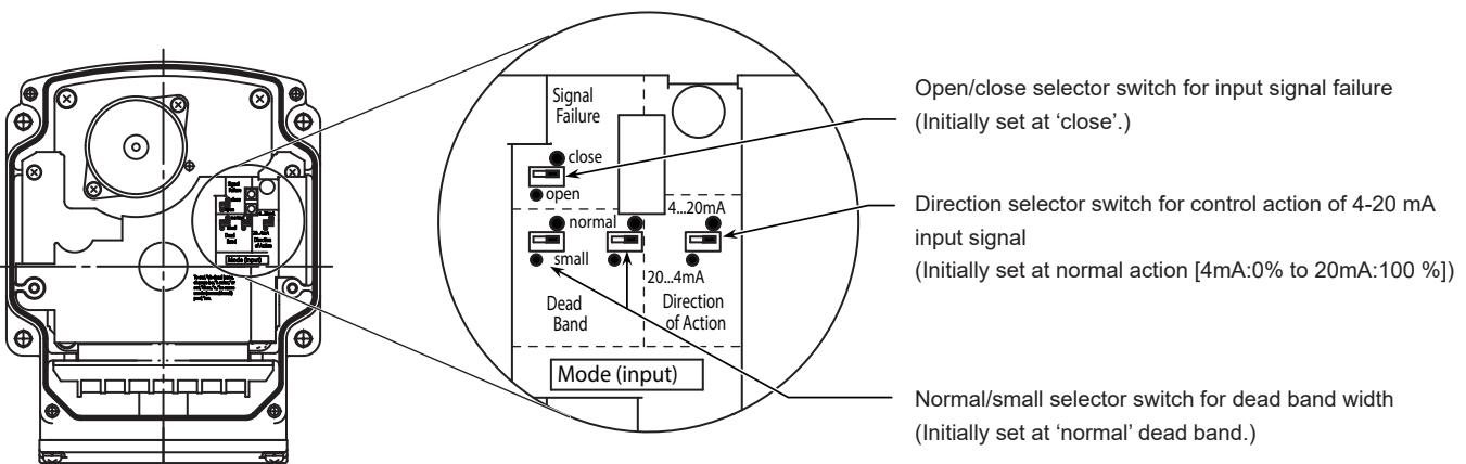
Figure 4 Selector switches
