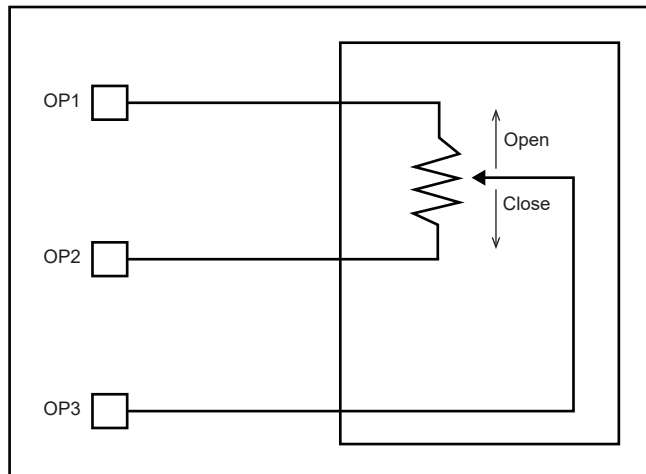
Figure 12 Internal connection of auxiliary potentiometer
