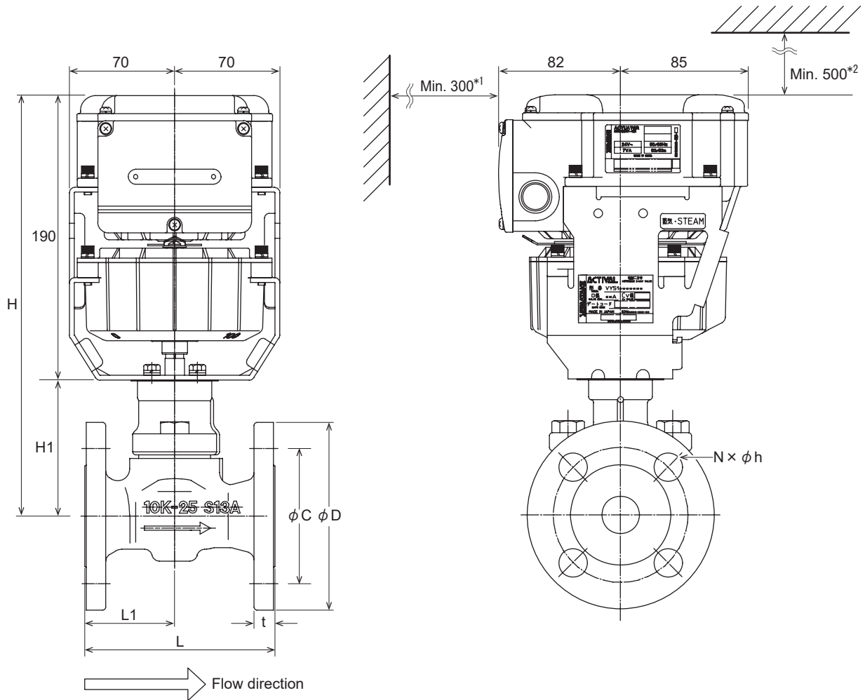
Figure 1 Dimensions (mm)
