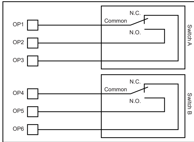
Figure 11 Internal connection of auxiliary switch
