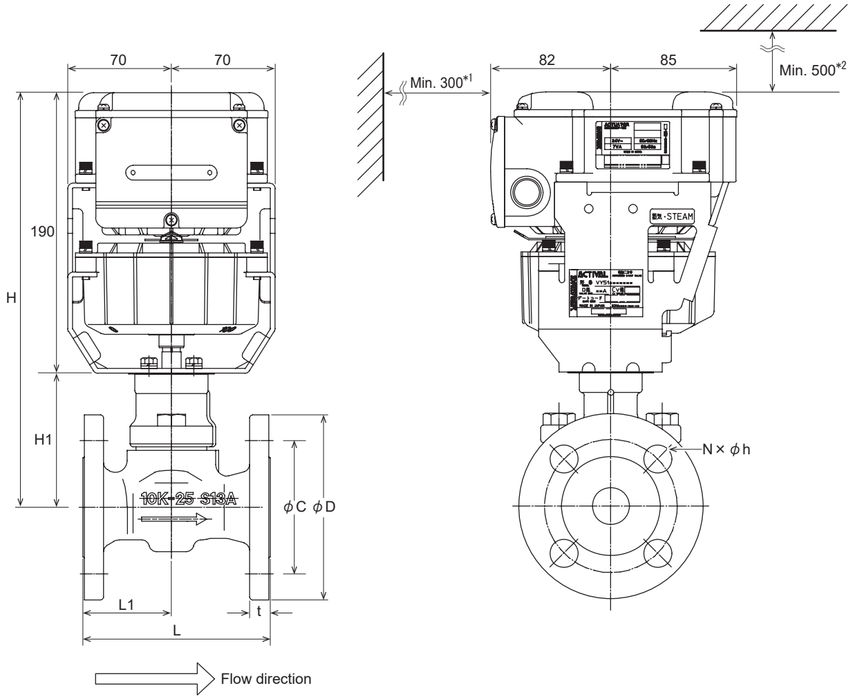
Figure2 Dimensions (mm)
