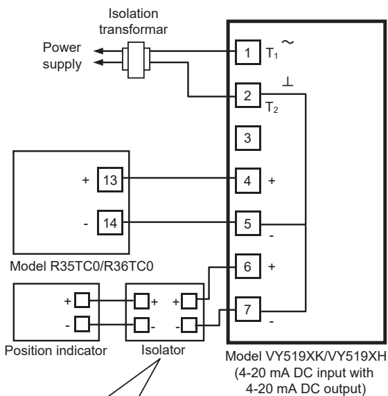
Connection to Model R35TC0/R36TC0
