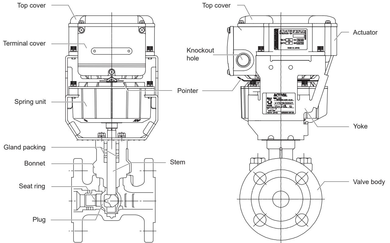
Figure3 Parts indication
