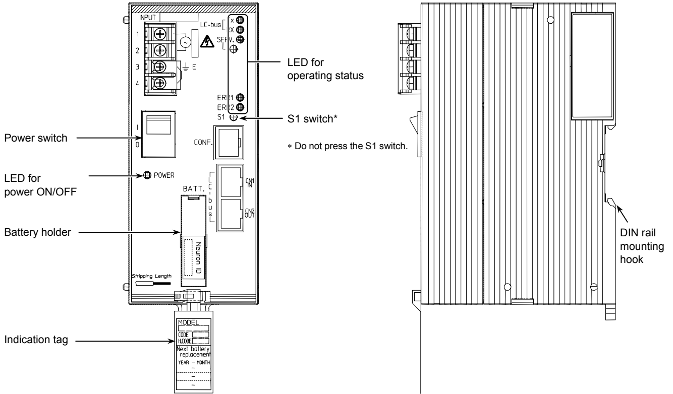
Figure 4. Parts identification
