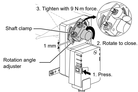
Figure 9. Complete installation of the actuator body
