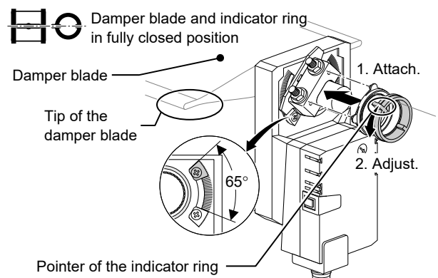
Figure 10. Attaching the position indicator ring
