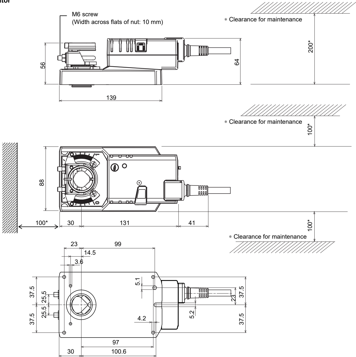
Figure 3. Dimensions (mm): Damper actuator
