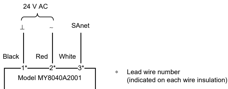
Figure 11. Lead wires connection
