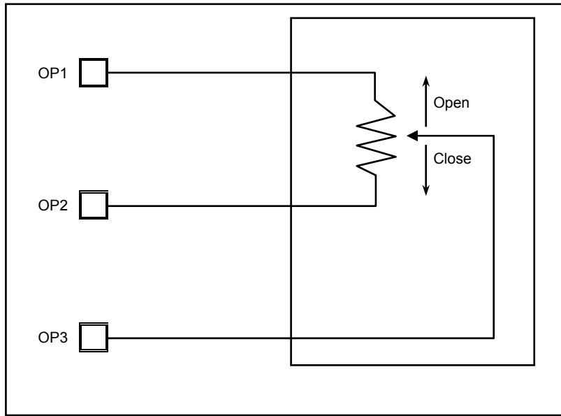
Figure 13. Internal connection of Part No. 83165275-001
