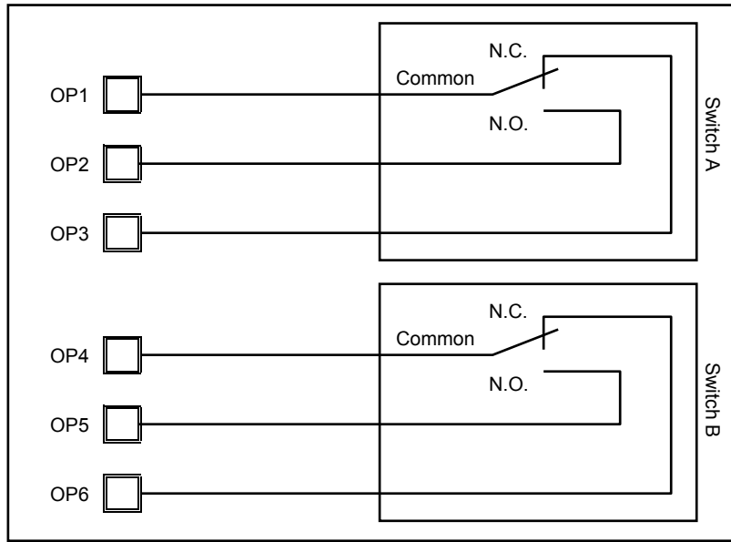
Figure 12. Internal connection of Part No. 83174063-101
