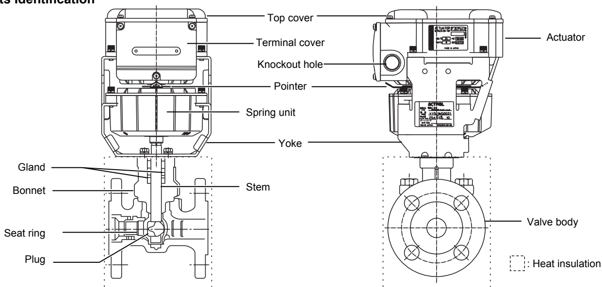
Figure 3. Parts identification
