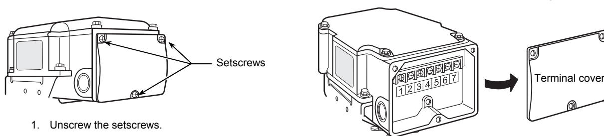
Figure 8. Terminal cover removal
