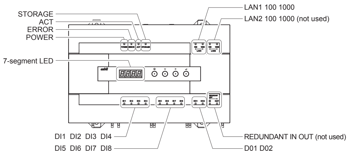
Figure 7. Indicator positions
