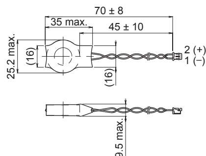
Figure 8. Outer shape of clock battery (unit: mm)
