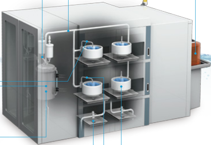
Single wafer type
