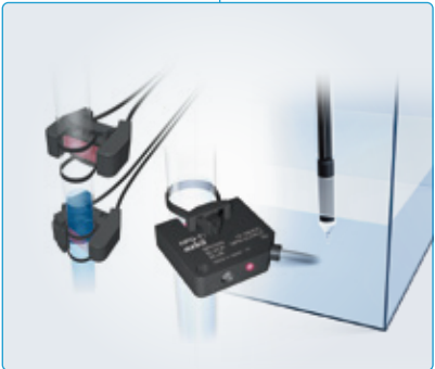
Liquid level detection [Product name] Pipe-mounted liquid level switches with built-in amplifier / Pipe-mounted / tank-inserted fiber-optic liquid level sensors [ Model No. ] HPQ-T_ / HPF-T032_ / HPF-T034 / HPF-D027 / HPF-D033 Application examples (Doc. No.) CP-PC-9000-002E
