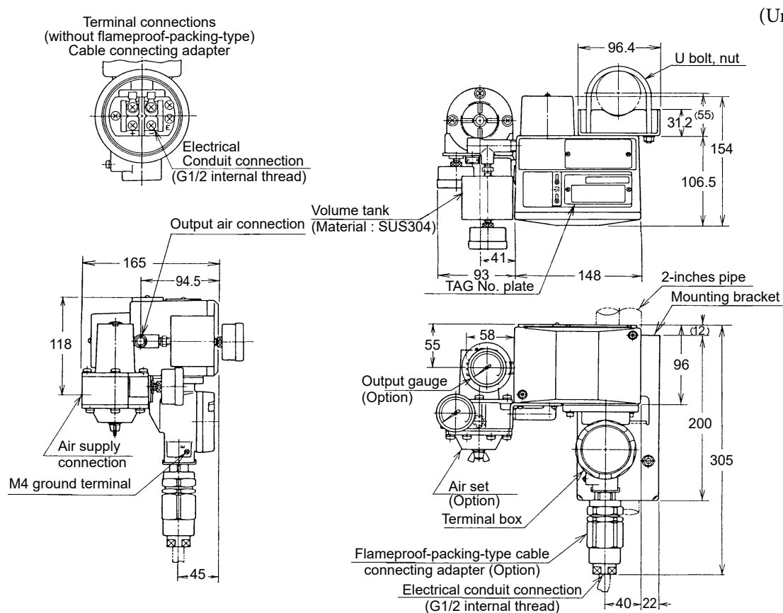
Figure 1. Dimension Drawing
