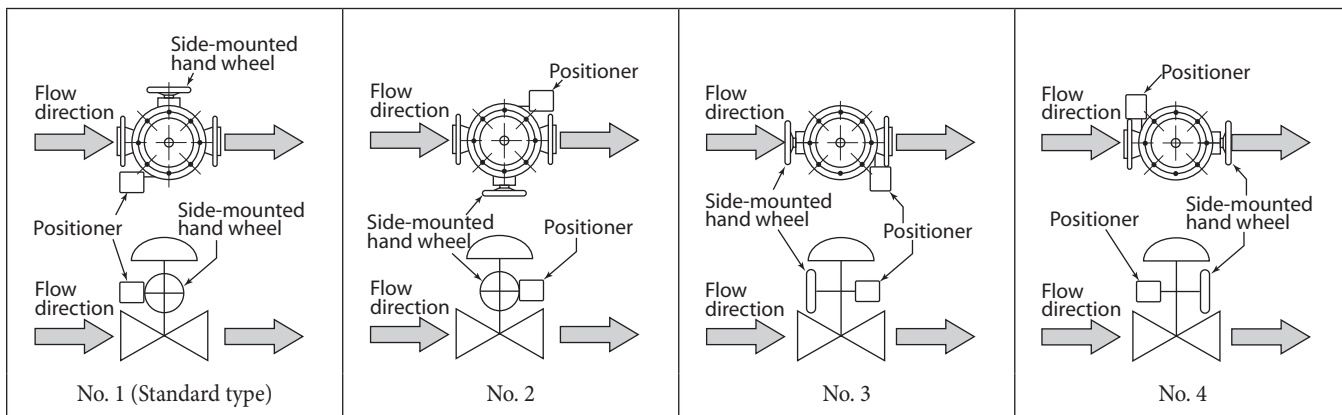
Figure 8. Actuator orientation
