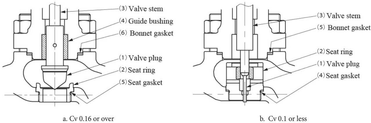
Figure 6. Structural drawing
