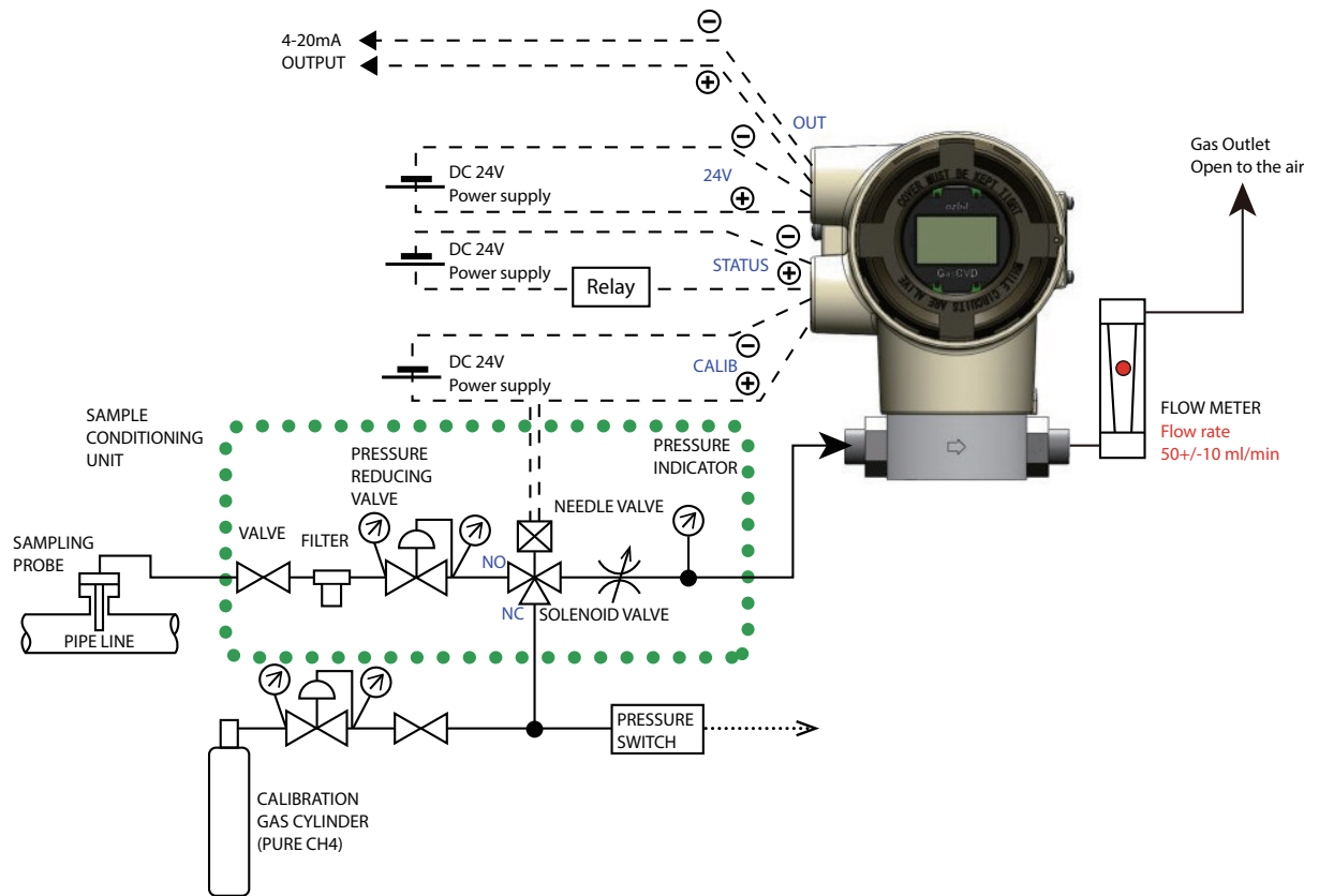
Figure 1. Example of recommended installation
