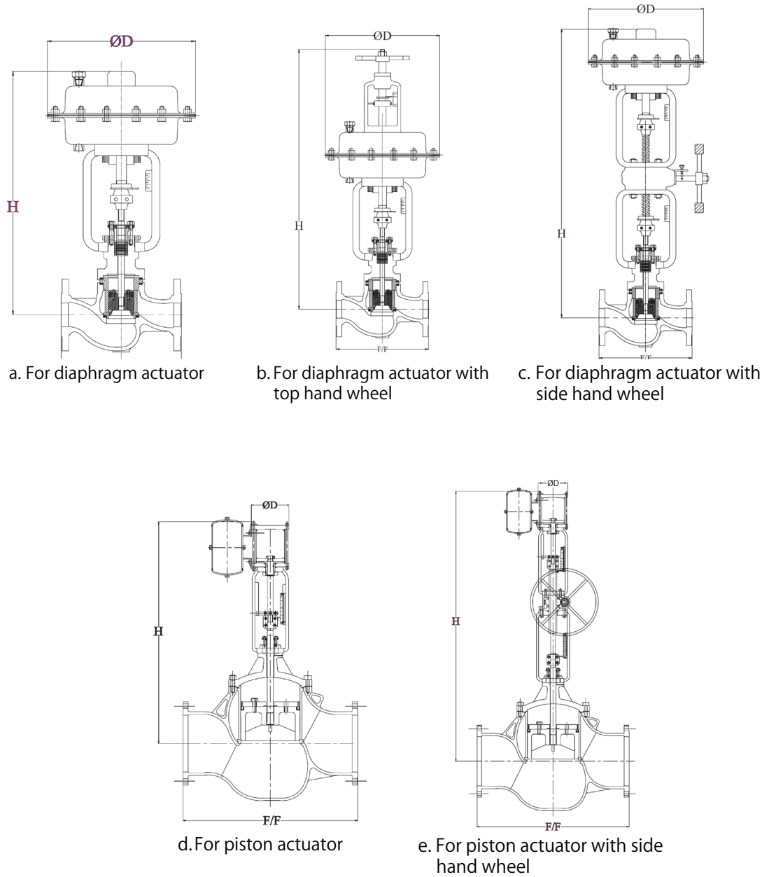
Figure1 Face-to-face and external dimensions
