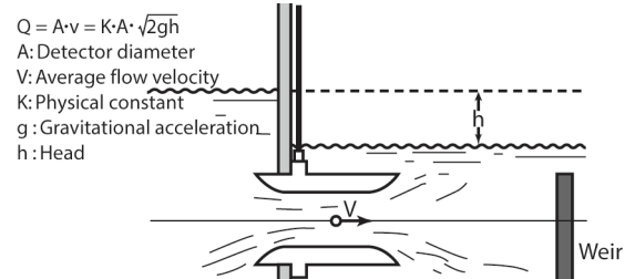
Figure 2. Principle of flow measurement with MagneW Flowmeter
