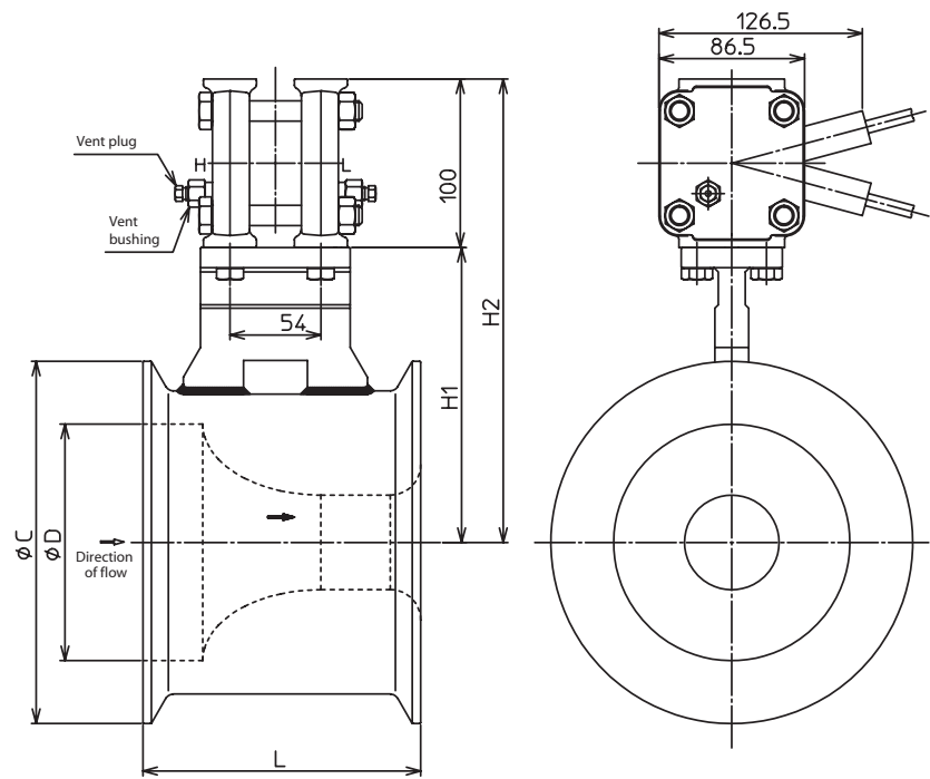
Horizontal piping from left to right (specification: 1)
