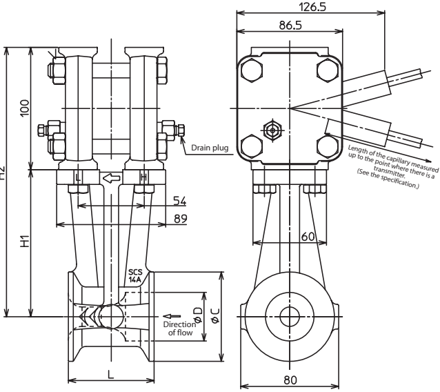
Horizontal piping from right to left (specification: 2)
