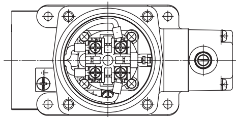
Wire routing
