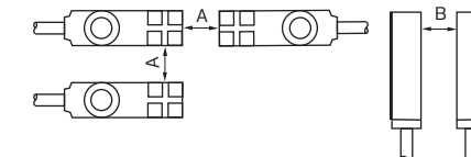
APM-C/D3 * 1(F)(-S)
